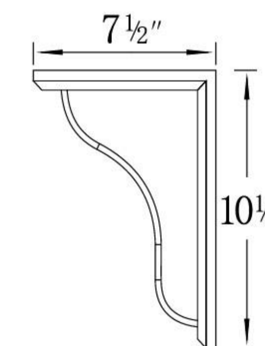
BRACKET
