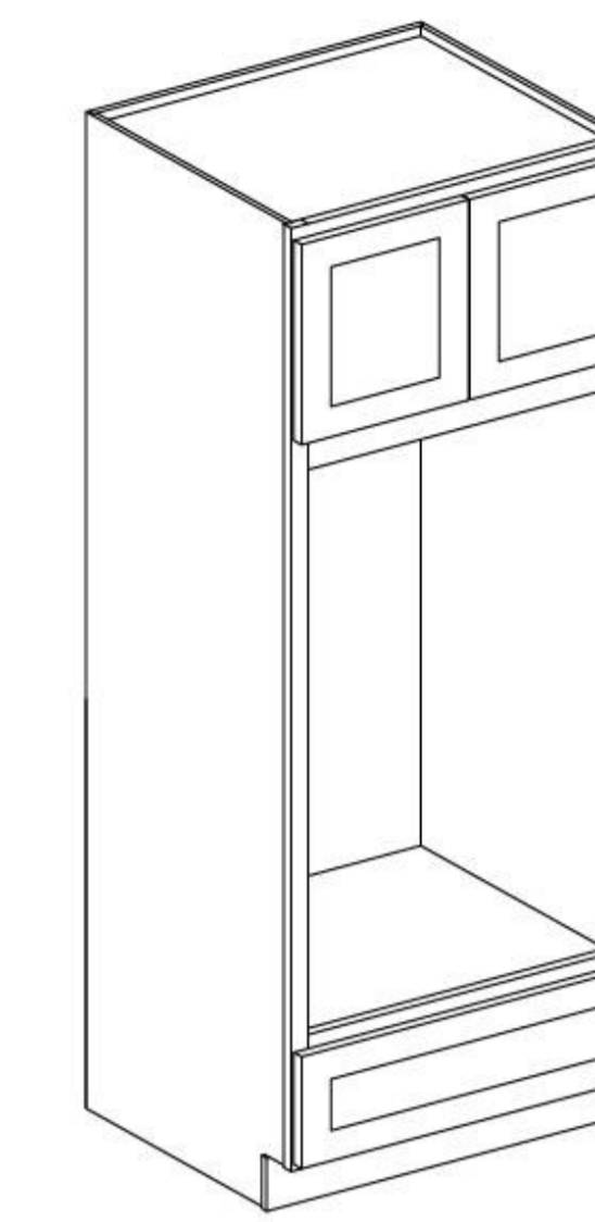
( Opening Size 28.5" W x 50" H ) OC31.584D OC31.590D OC31.596D OC3384D OC3390D OC3396D
